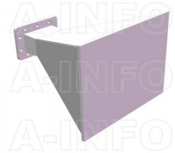
LB-284-15-ASPO Standard Gain Horn Antenna 2.6-3.95GHz 15dB Gain Rectangular Waveguide Interface
