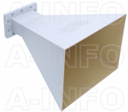
LB-284-15-A Standard Gain Horn Antenna 2.6-3.95GHz 15dB Gain Rectangular Waveguide Interface
